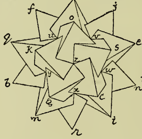
V. Icosa-hedron
